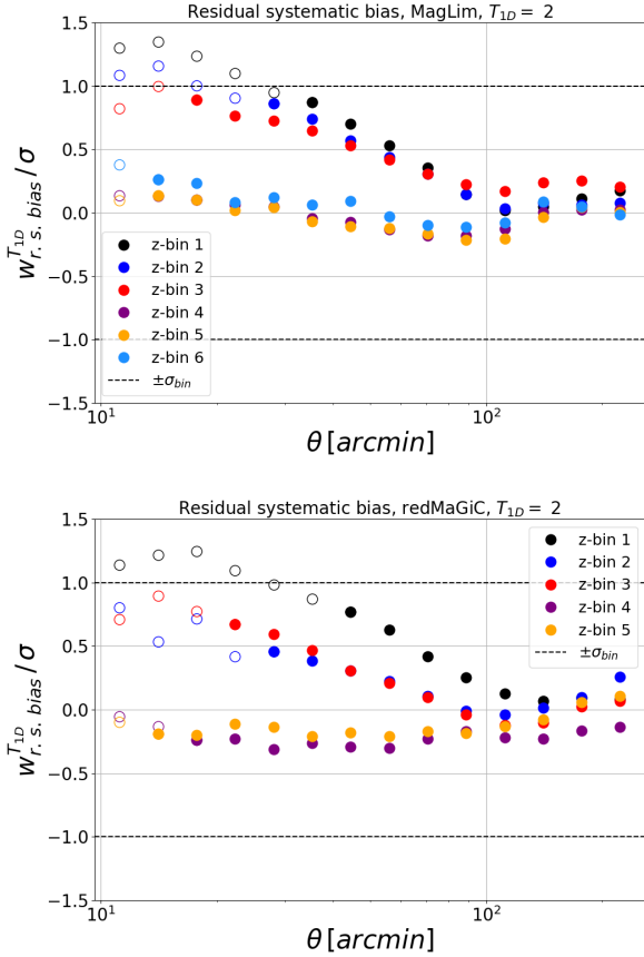
Figure 6. Residual systematic bias, w_{r,s}^{T_{1D}}(\theta) , for MAGLIM (top panel) and REDMAGIC (bottom panel) relative to the w(\theta) error from the unaltered COSMOLIKE covariance diagonal. The empty dots represent the scales excluded at each bin. Both samples show similar trends: the highest redshift bins present lower biases, while the lowest ones show important levels of undercorrection at the smallest scales. On the other hand, the largest scales are recovered nearly unbiased. Since the \chi^2 of the total residual bias in all bins is higher than 3, we add a systematic term to the covariance matrix to marginalise over this effect.
