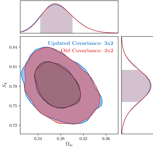
FIG. 21. Constraints on \Omega_m and S_8 when updating the covariance matrix after initial unblinding and using the means of the posteriors generated when using the old covariance matrix.
