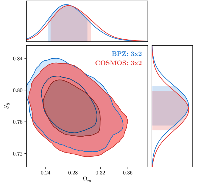
FIG. 20. Constraints on \Omega_m and S_8 when using the shifted BPZ redshift distributions as the default for n_s^i(z) , compared with those obtained when using the COSMOS redshift distribution, which have different shape, as seen in Figure 4 of [83].
